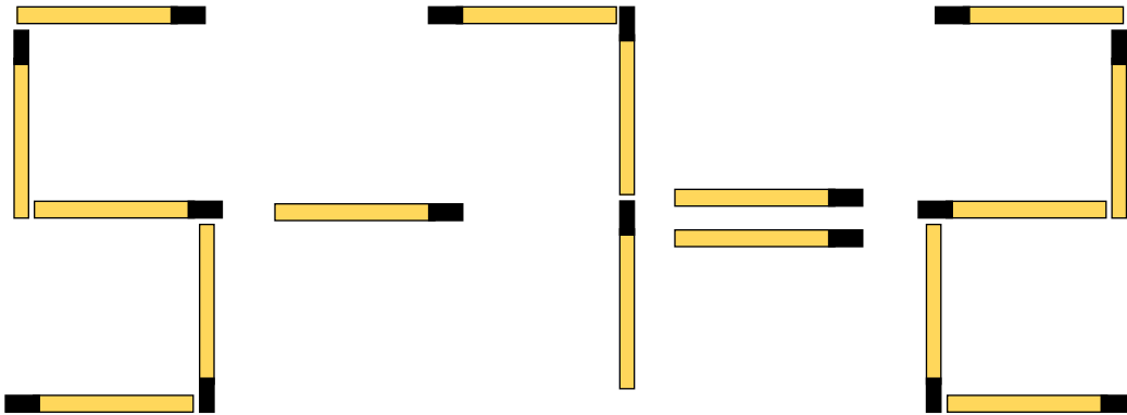
Equation 1
