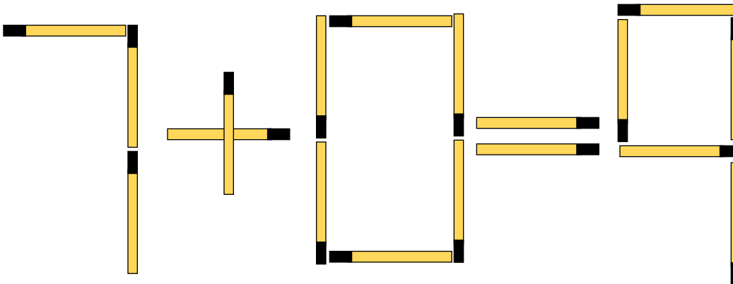
Equation 2
